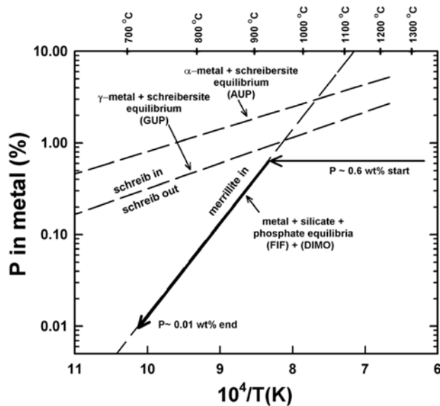
Fig. 16. Modelled evolution of P content in the metal of Portales Valley as a function of temperature. In principle, the P content in metal under subsolidus conditions could be controlled either by metal-silicate-phosphate (FIF and DIMO) equilibria or metal-phosphide equilibria (GUP or AUP), but our analysis suggests that for the range of P contents likely present in PV metal ( P \leq 0.6 wt%), equilibria with silicates and the formation of phosphate likely controlled the evolution of P content in metal.
